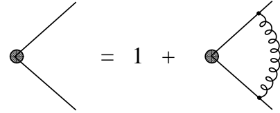
FIG. 2: Diagrammatic illustration of the integral equation for the Coulomb form factor f represented by the fat dot with two entries for external legs.
