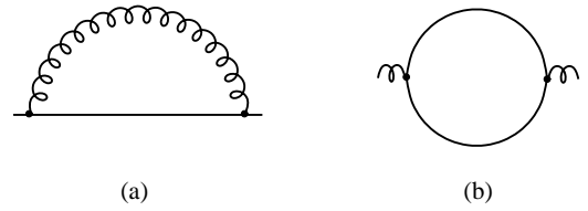
FIG. 1: (a) The ghost self-energy in the rainbow ladder approximation. The full (wavy) line represents the full ghost (gluon) propagator. (b) Ghost loop contribution to the gluon self-energy.
